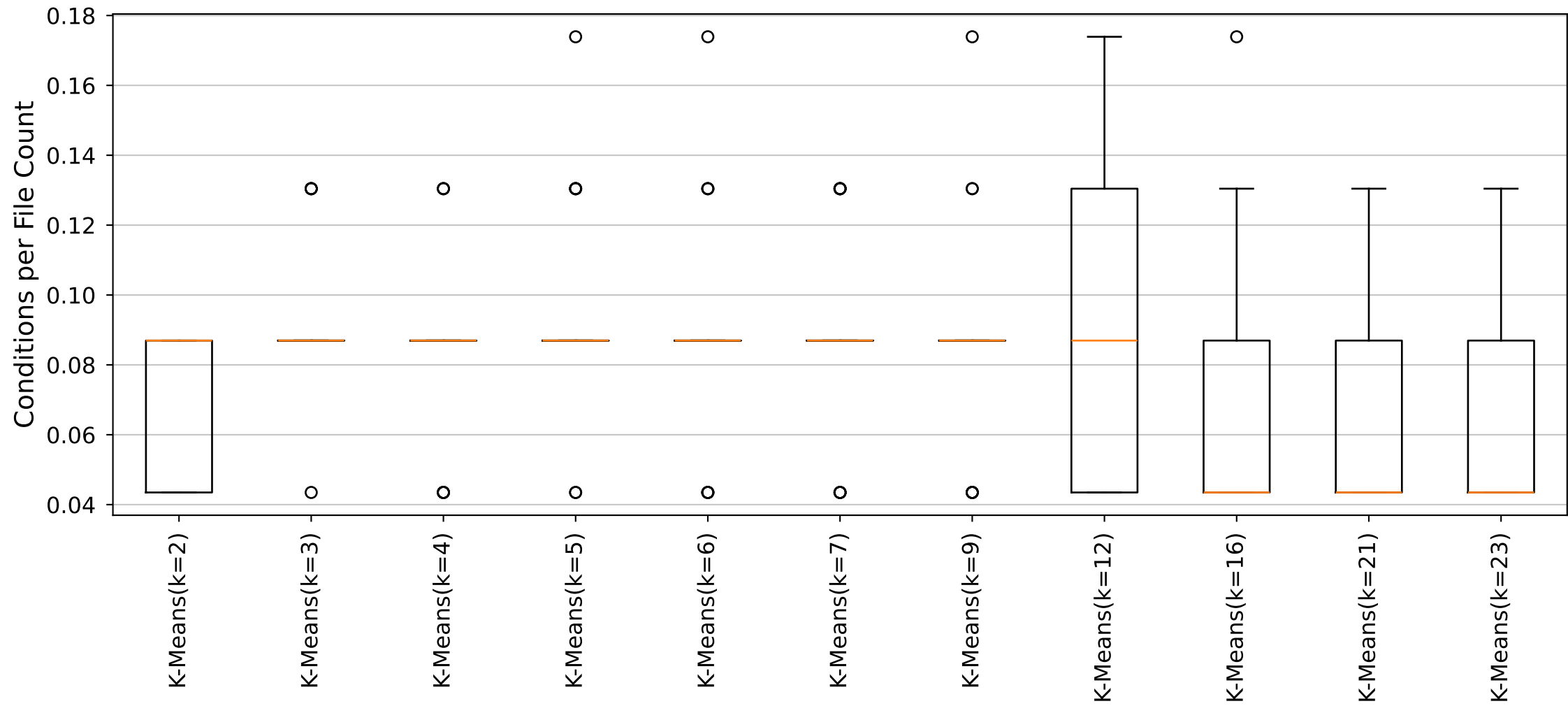
YARA Rules Conditions per File Count Distribution (Cluster6_Size23 dataset)
